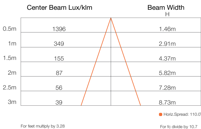
Illuminance at a distance
